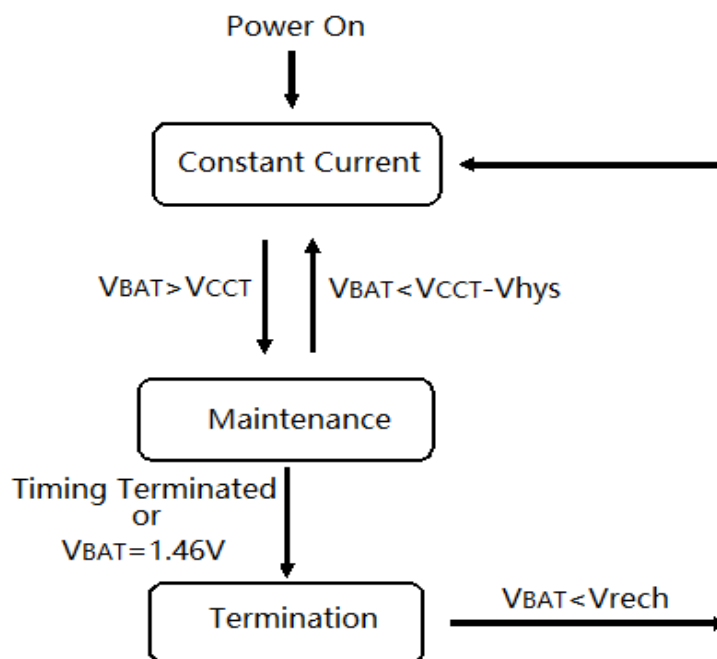
Figure 3 Charging Flow
